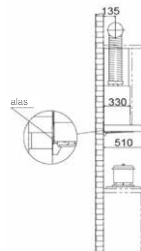
Gambar 2. Diagram Instalasi
